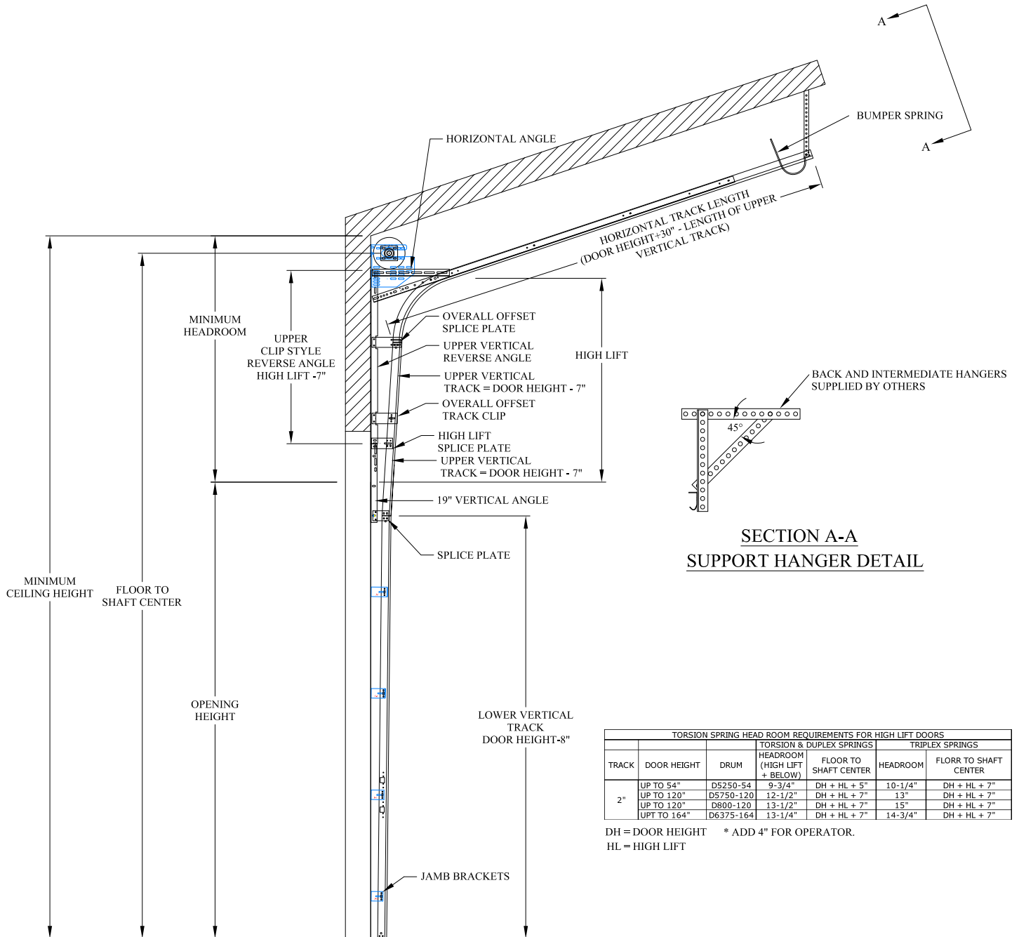
HIGH LIFT STANDARD BRACKET MOUNT TRACK SET DETAIL FOLLOW THE ROOF PITCH
