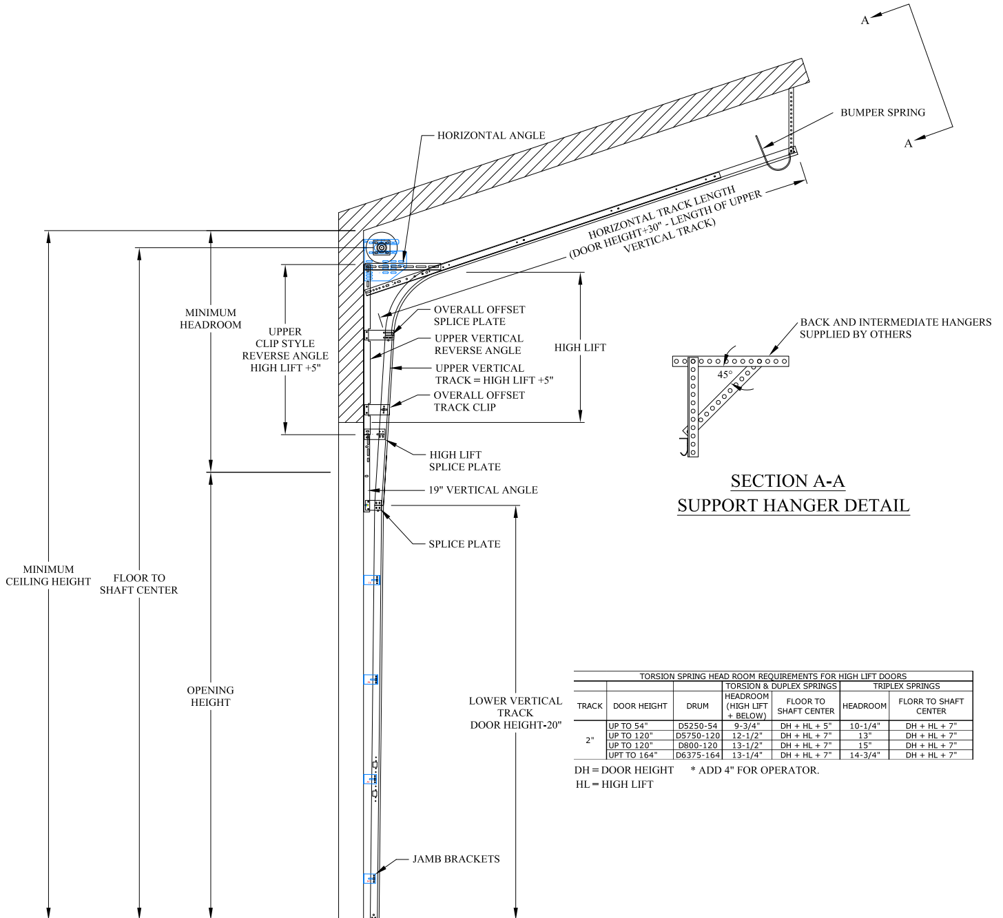
HIGH LIFT BREAKAWAY BRACKET MOUNT TRACK SET DETAIL FOLLOW THE ROOF PITCH
