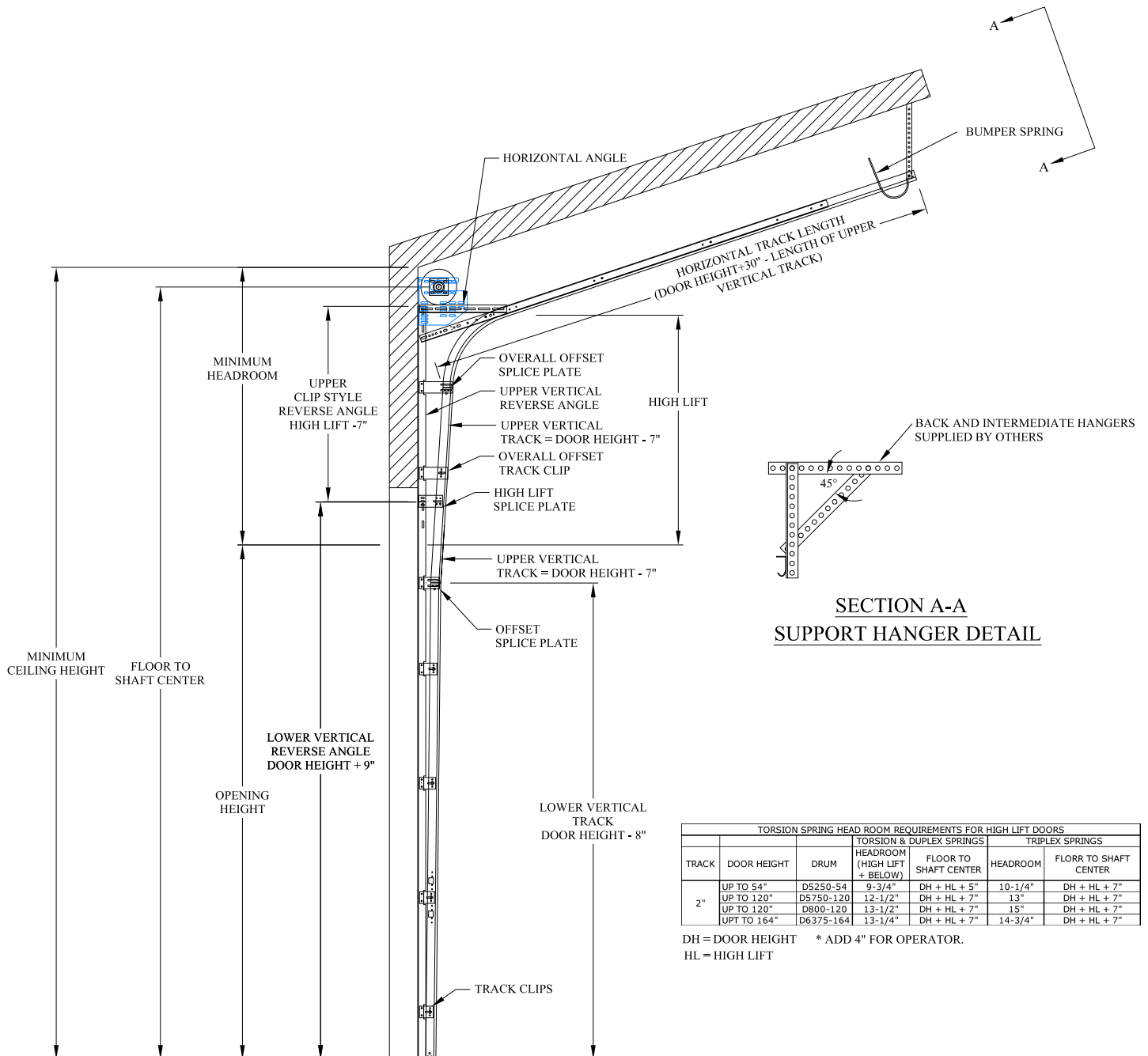
HIGH LIFT STANDARD ANGLE MOUNT TRACK SET DETAIL FOLLOW THE ROOF PITCH
