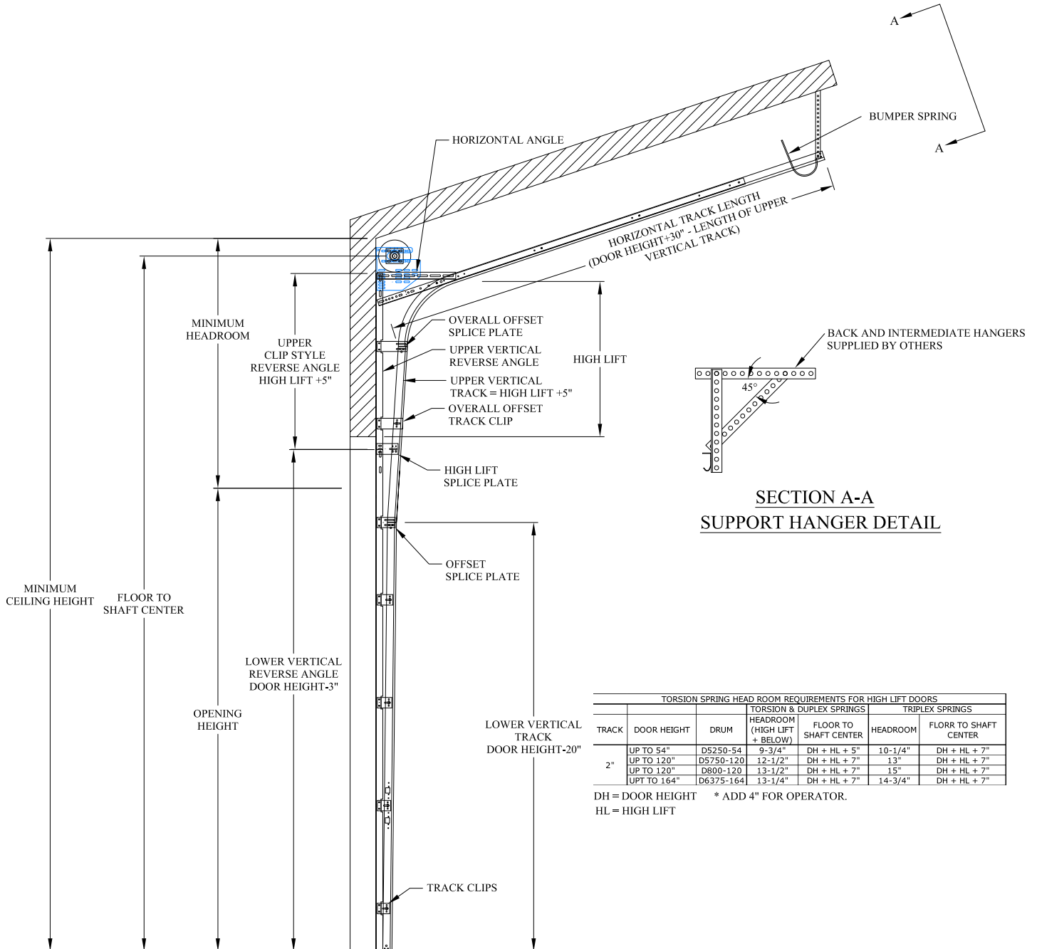
HIGH LIFT BREAKAWAY ANGLE MOUNT TRACK SET DETAIL FOLLOW THE ROOF PITCH
