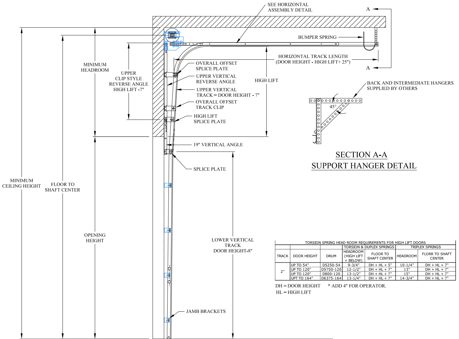
HIGH LIFT STANDARD BRACKET MOUNT TRACK SET DETAIL
