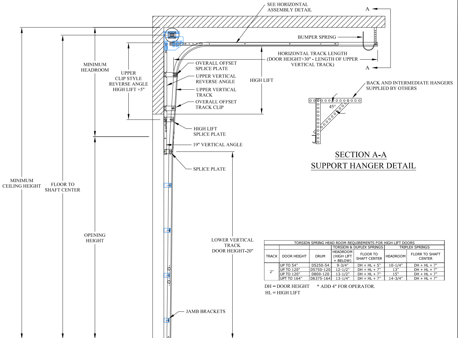
HIGH LIFT BREAKAWAY BRACKET MOUNT TRACK SET DETAIL
