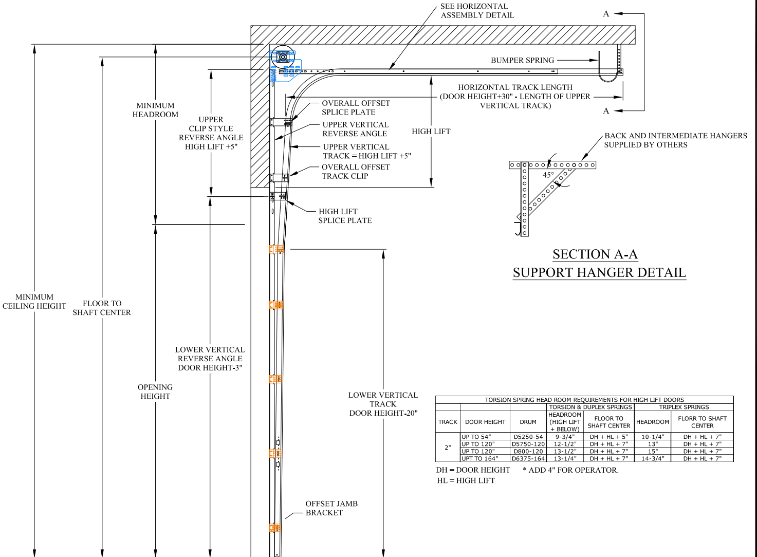
HIGH LIFT BREAKAWAY REVERSE WITH JAMB BRACKET MOUNT TRACK SET DETAIL
