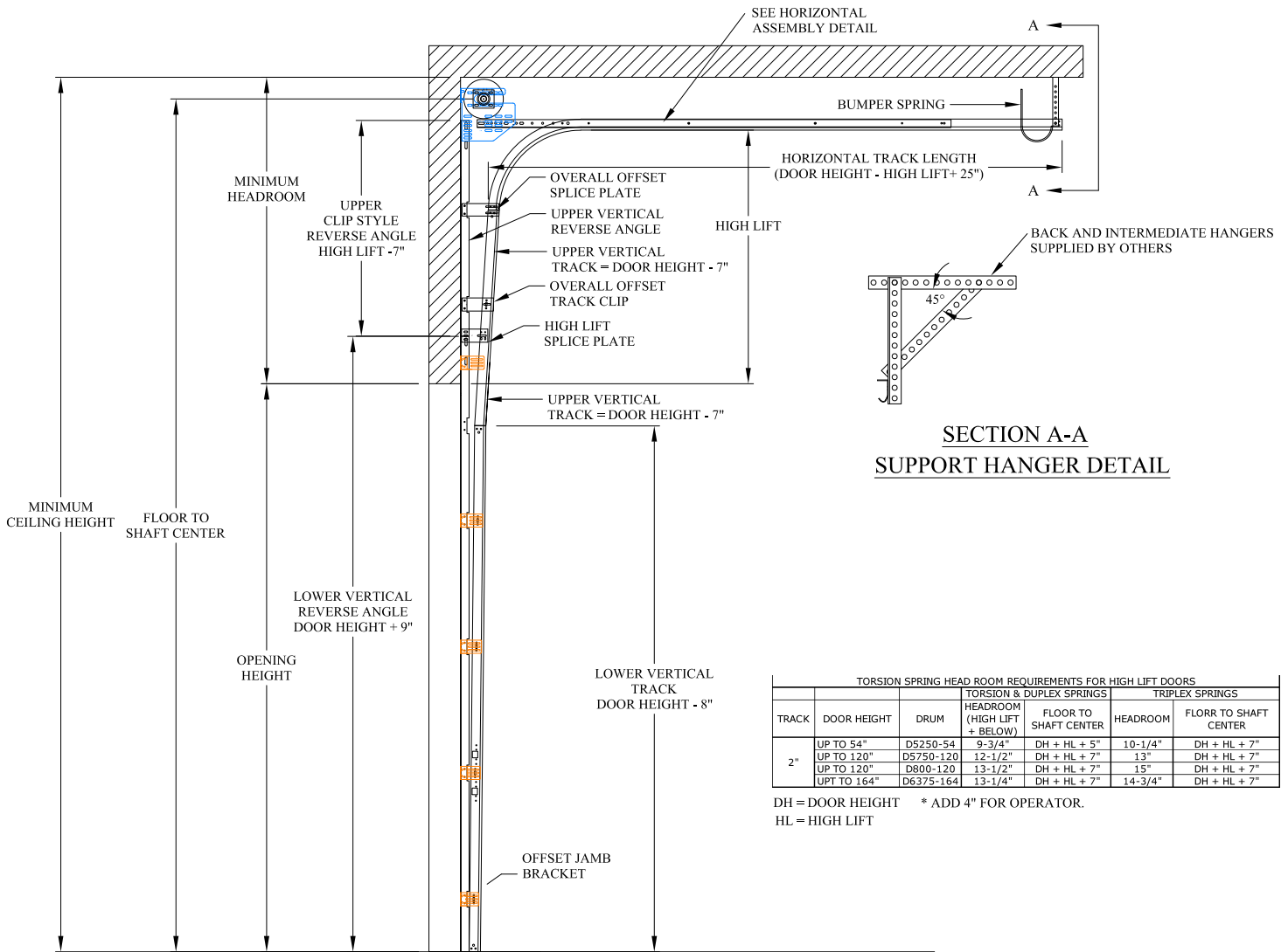
HIGH LIFT STANDARD REVERSE WITH JAMB BRACKET MOUNT TRACK SET DETAIL
