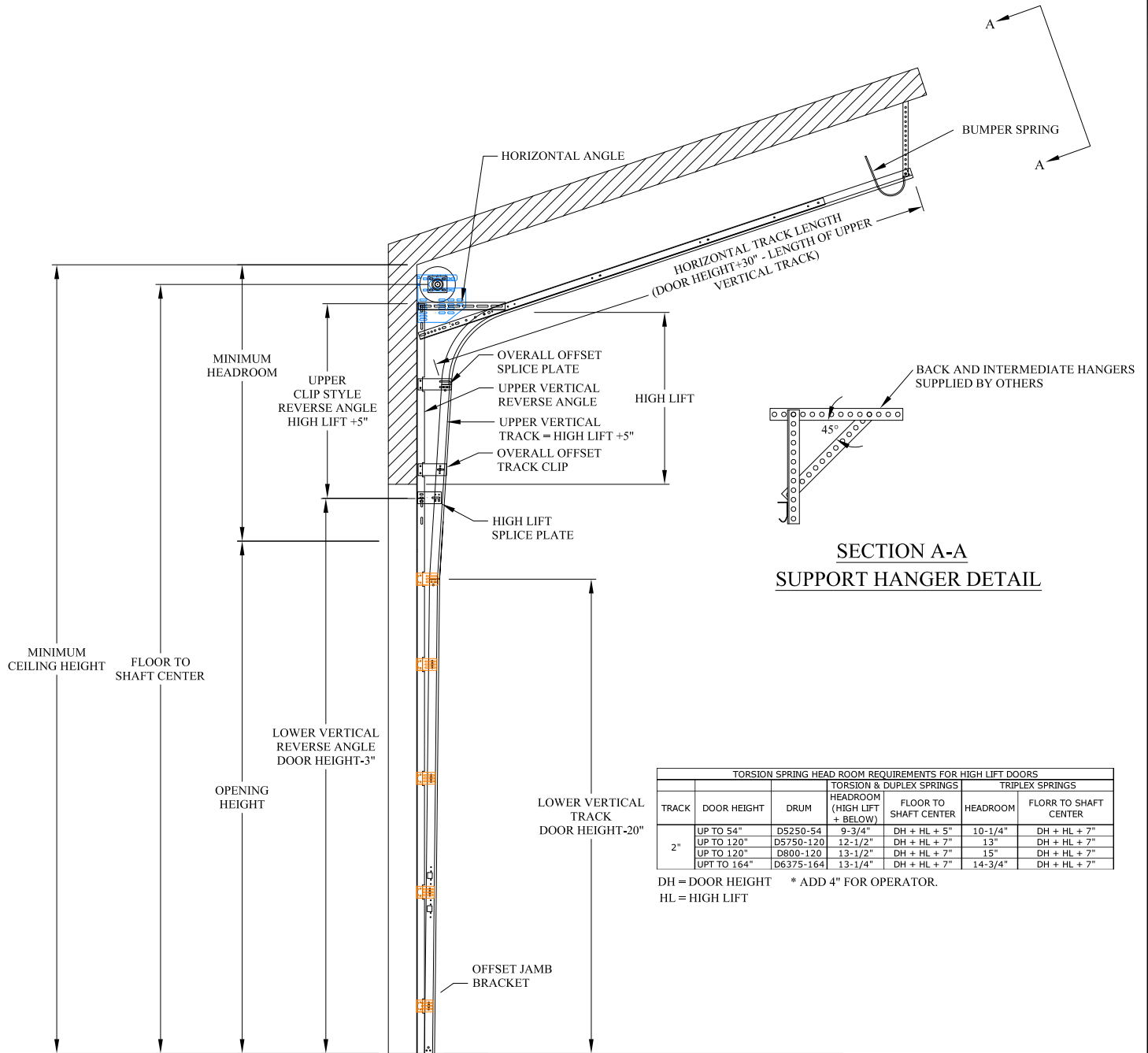
HIGH LIFT BREAKAWAY REVERSE WITH JAMB BRACKET MOUNT TRACK SET DETAIL FOLLOW THE ROOF PITCH
