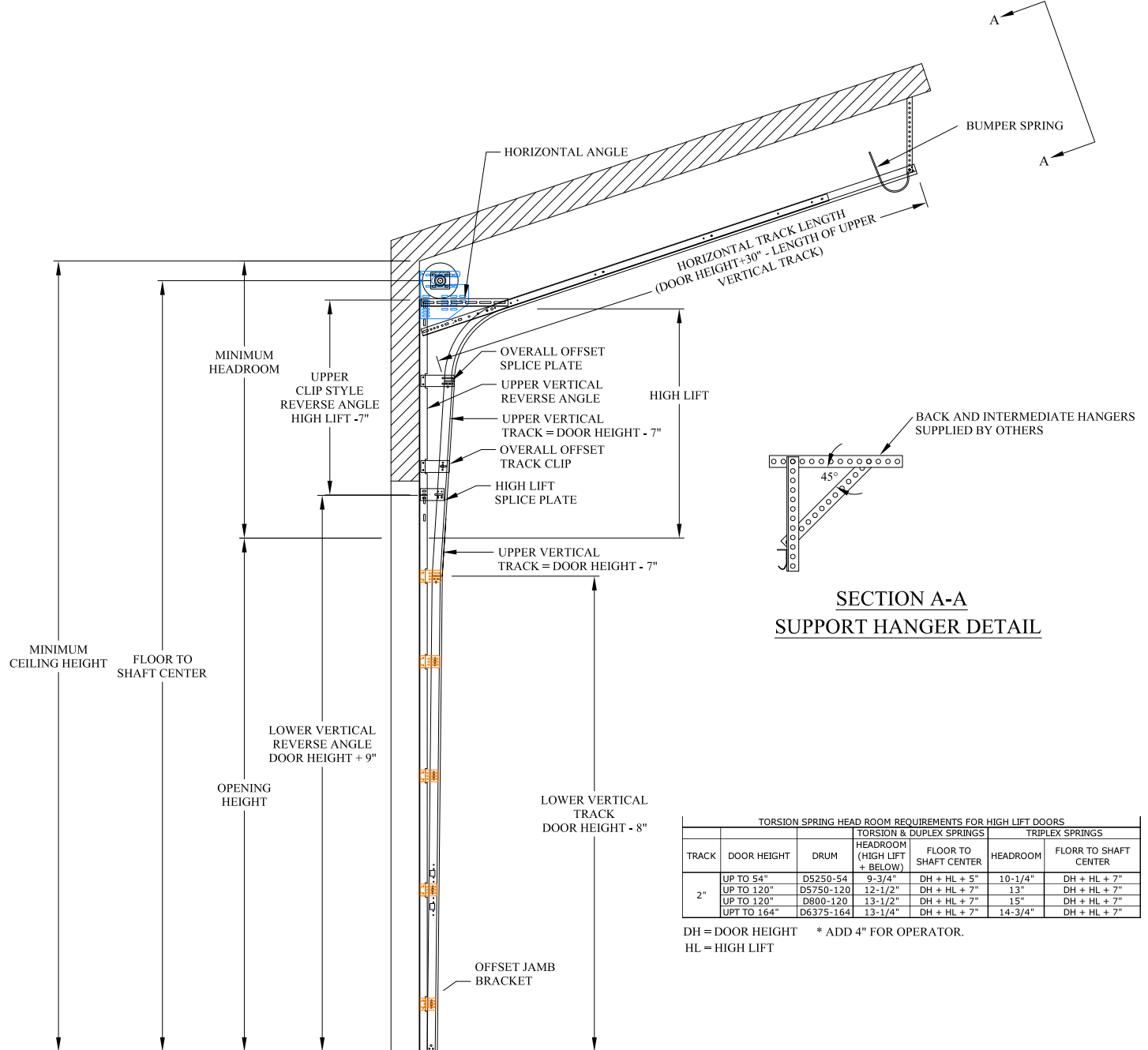
HIGH LIFT STANDARD REVERSE WITH JAMB BRACKET MOUNT TRACK SET DETAIL FOLLOW THE ROOF PITCH
