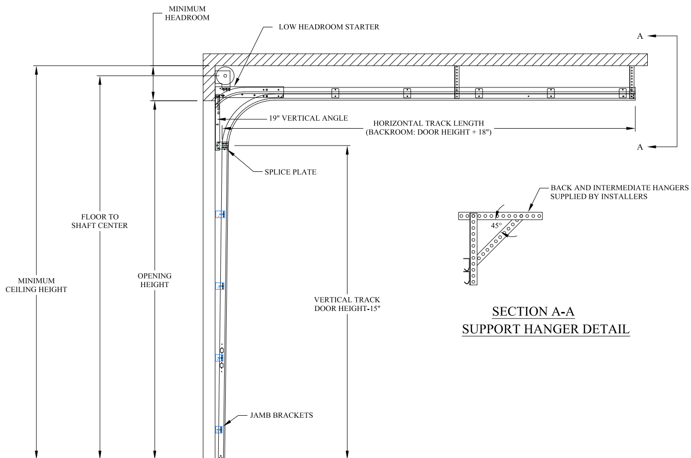
LOW HEADROOM TO THE FRONT BRACKET MOUNT TRACK SET DETAIL
