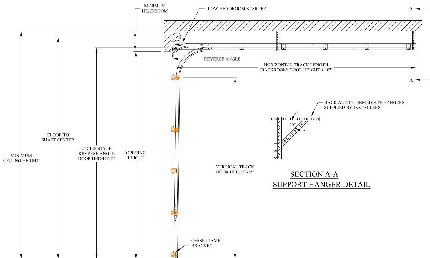
LOW HEADROOM TO THE FRONT REVERSE JAMB BRACKET MOUNT TRACK SET DETAIL
