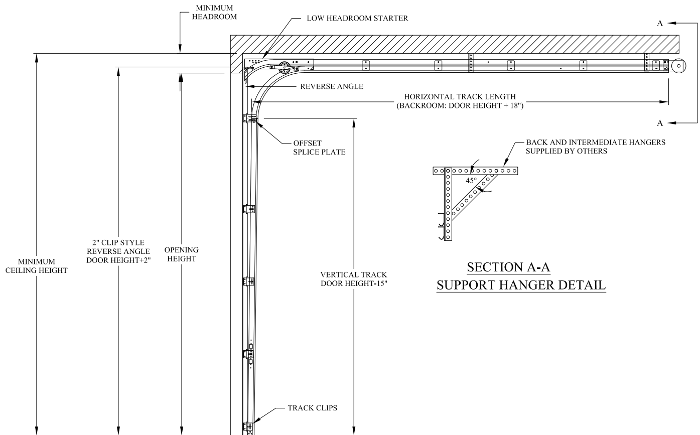
LOW HEADROOM TO THE REAR ANGLE MOUNT TRACK SET DETAIL
