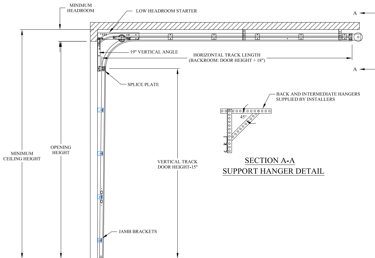
LOW HEADROOM TO THE REAR BRACKET MOUNT TRACK SET DETAIL
