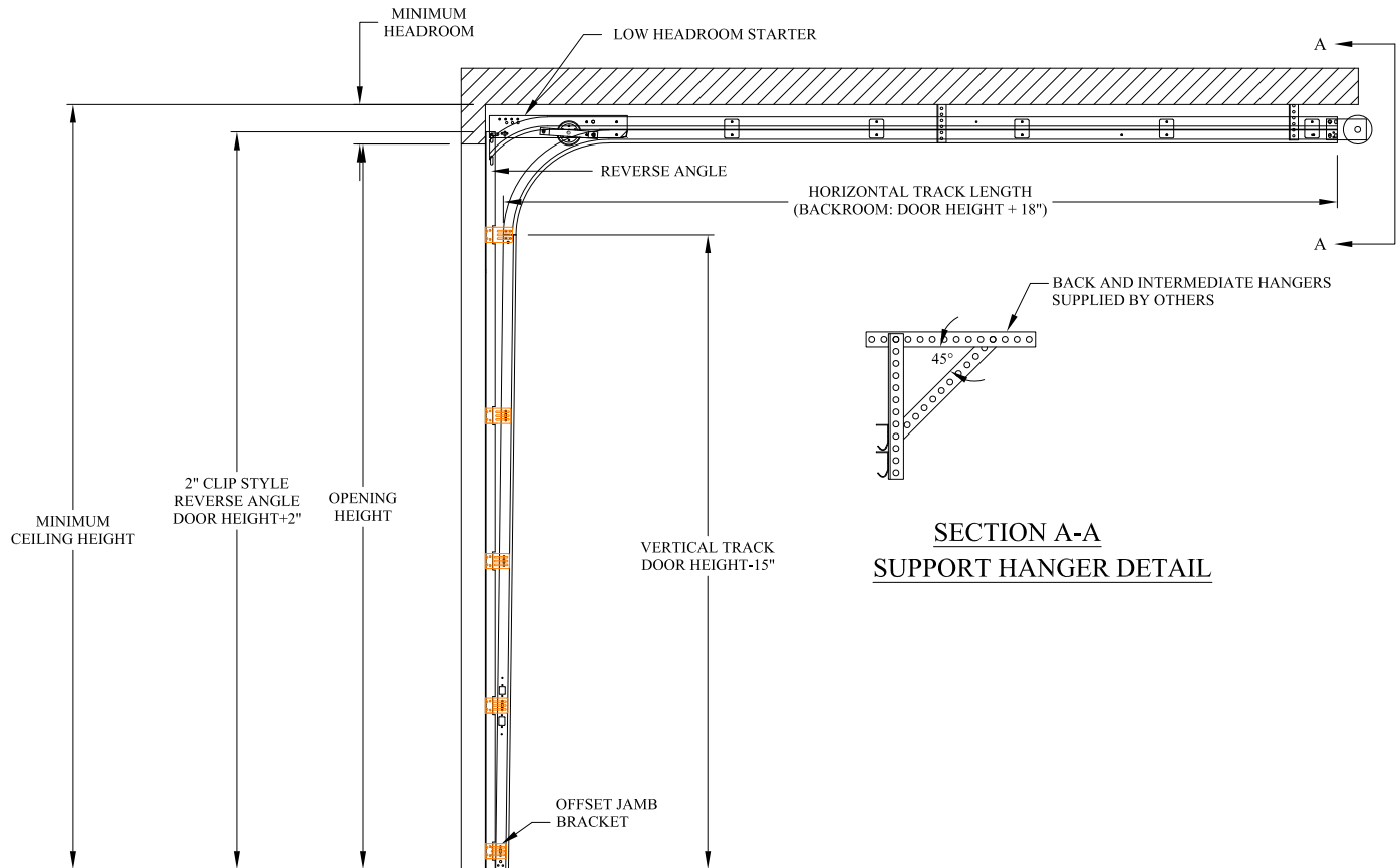
LOW HEADROOM TO THE REAR REVERSE JAMB BRACKET MOUNT TRACK SET DETAIL
