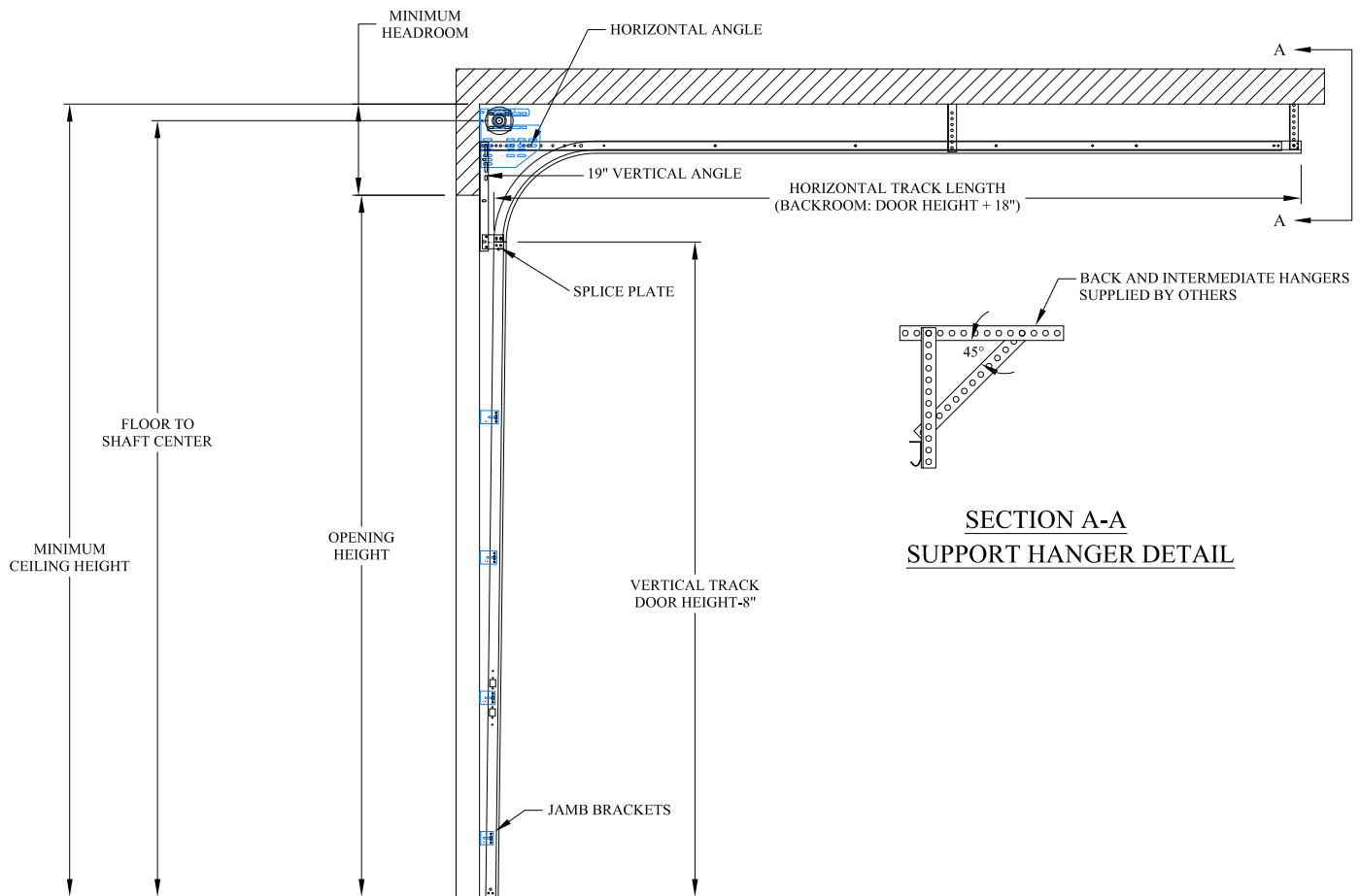
STANDARD LIFT BRACKET MOUNT TRACK SET DETAIL
