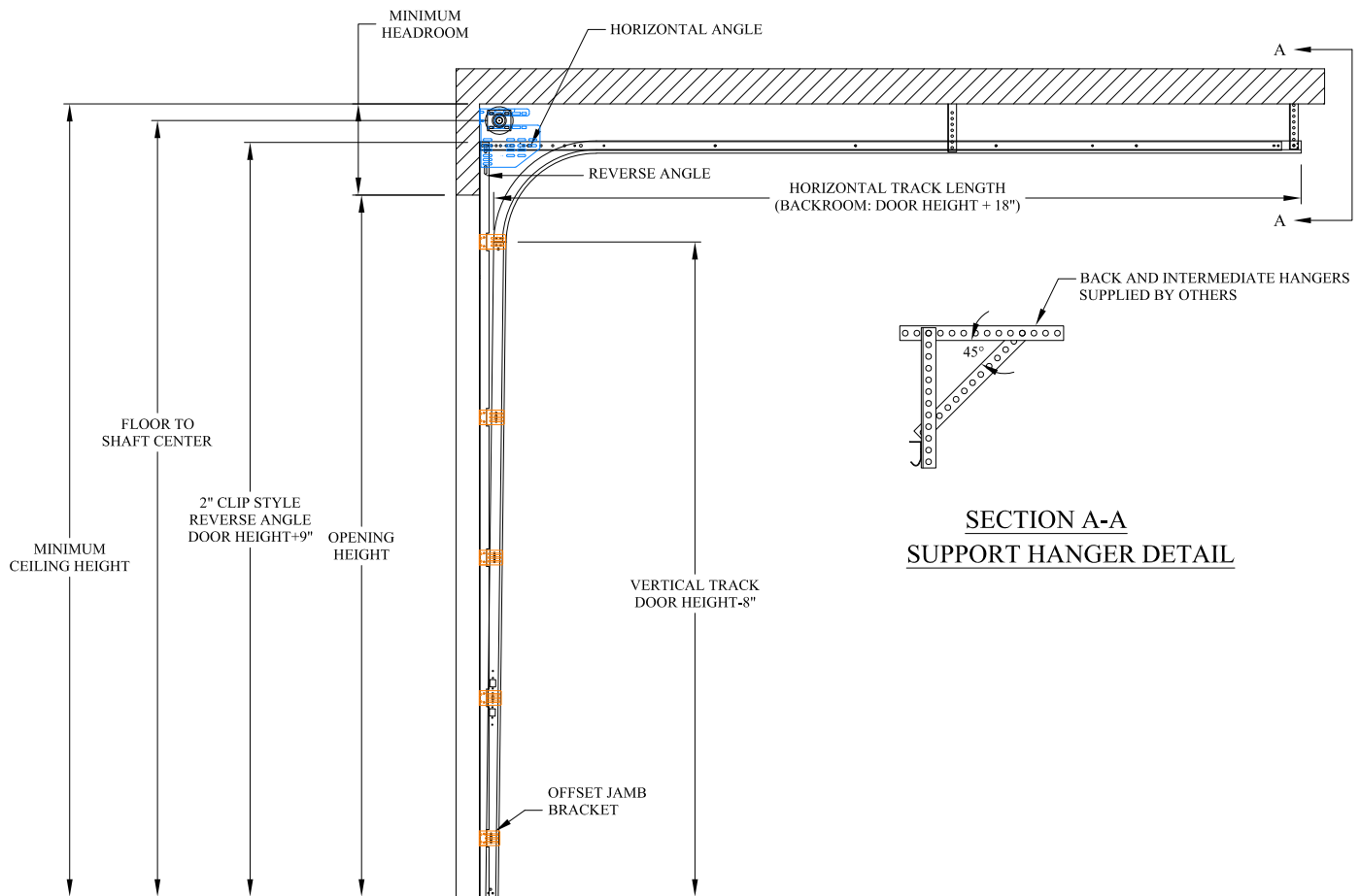
STANDARD LIFT REVERSE JAMB BRACKET MOUNT TRACK SET DETAIL
