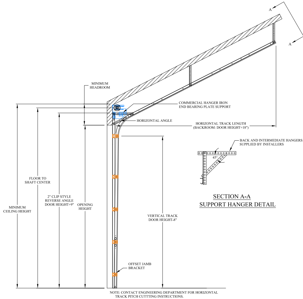
STANDARD LIFT REVERSE JAMB BRACKET MOUNT TRACK SET DETAIL FOLLOW THE ROOF PITCH
