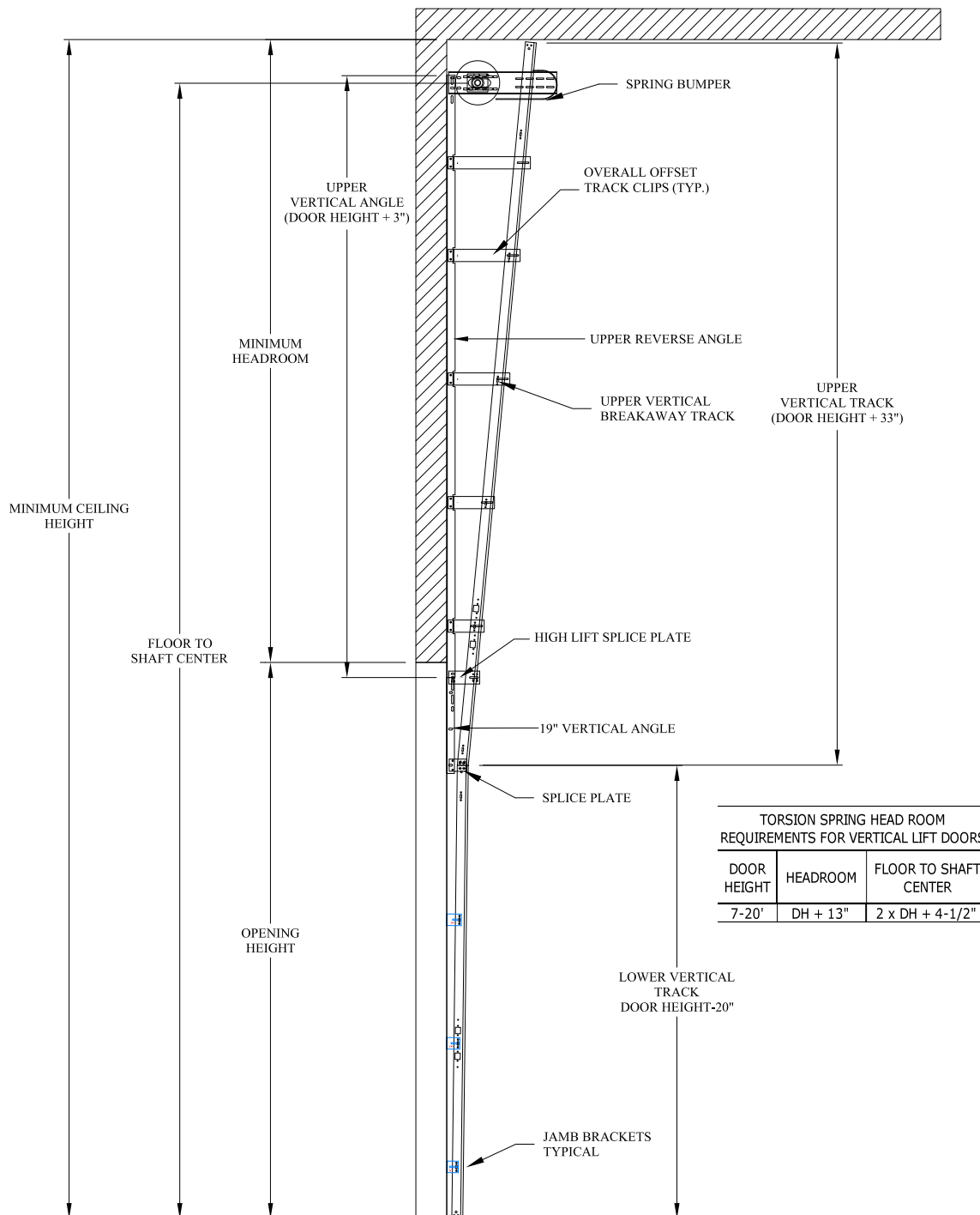
BREAKAWAY VERTICAL LIFT BRACKET MOUNT TRACK SET DETAIL
