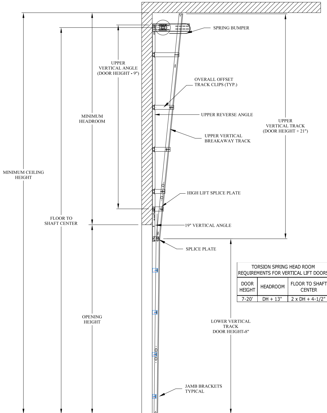
STANDARD VERTICAL LIFT BRACKET MOUNT TRACK SET DETAIL
