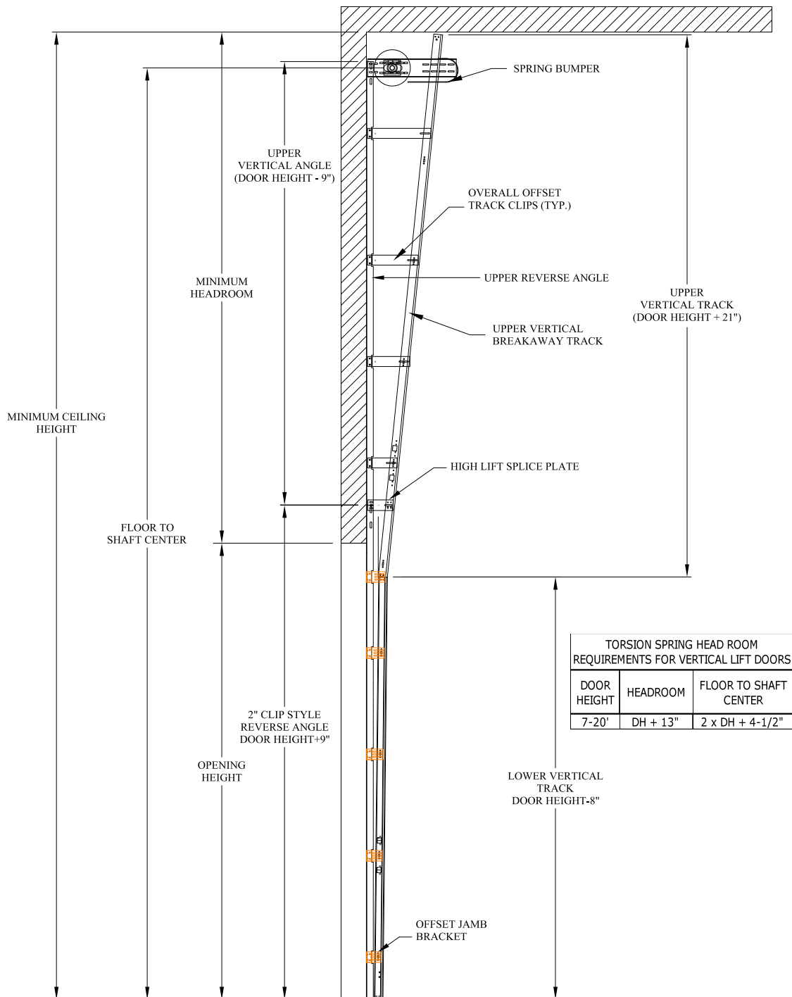
STANDARD VERTICAL LIFT REVERSE JAMB BRACKET MOUNT TRACK SET DETAIL
