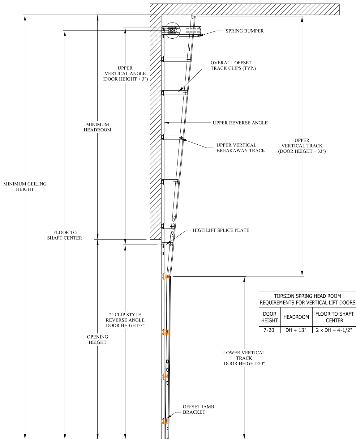
BREAKAWAY VERTICAL LIFT REVERSE JAMB BRACKET MOUNT TRACK SET DETAIL
